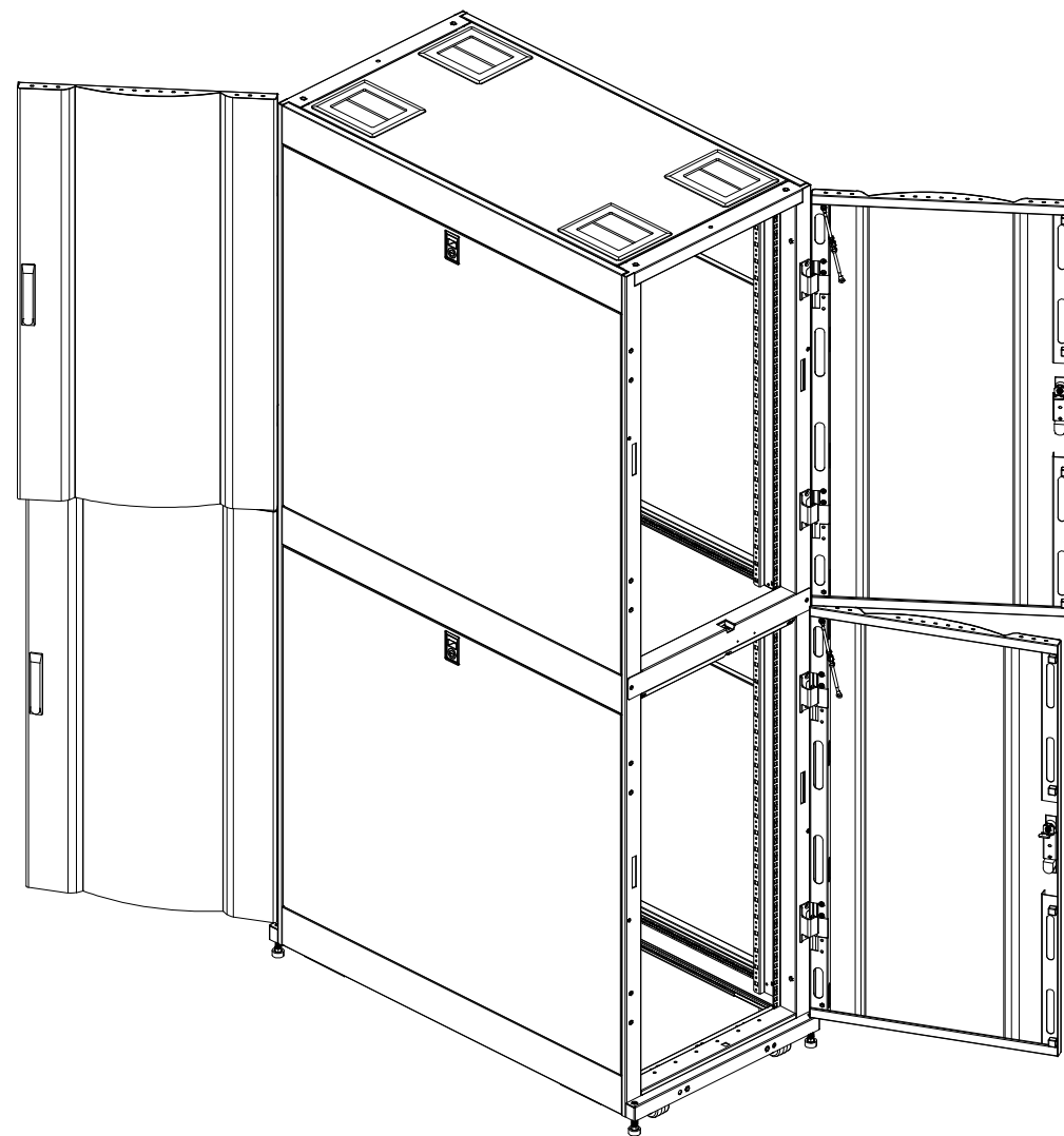
FRONT VIEW (OPEN DOORS)
